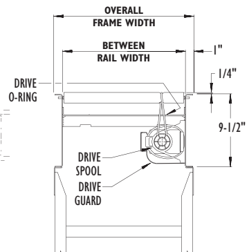
SECTION "X-X"
